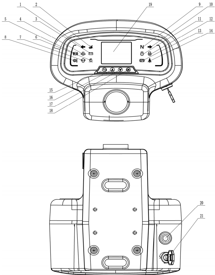
Figure 12-2 Dashboard assy 293933510008
