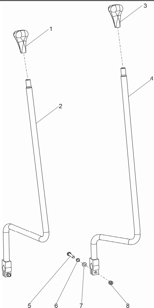
Figure 7-2 Variable speed control assembly
