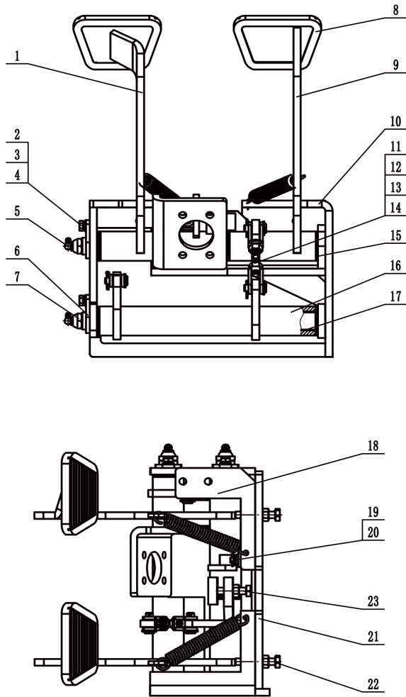
Figure 8-2-1 Brake Micro Assembly 293911511003
